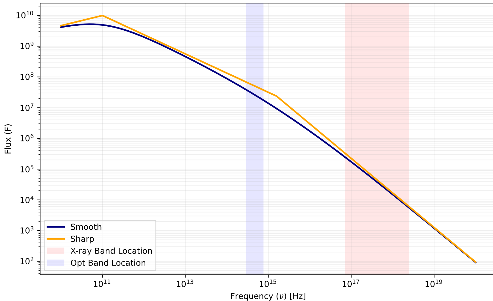
Smooth vs. Sharp Spectral Model ( p = 2.25 , \nu_c = 1.585\text{e}+15 )
