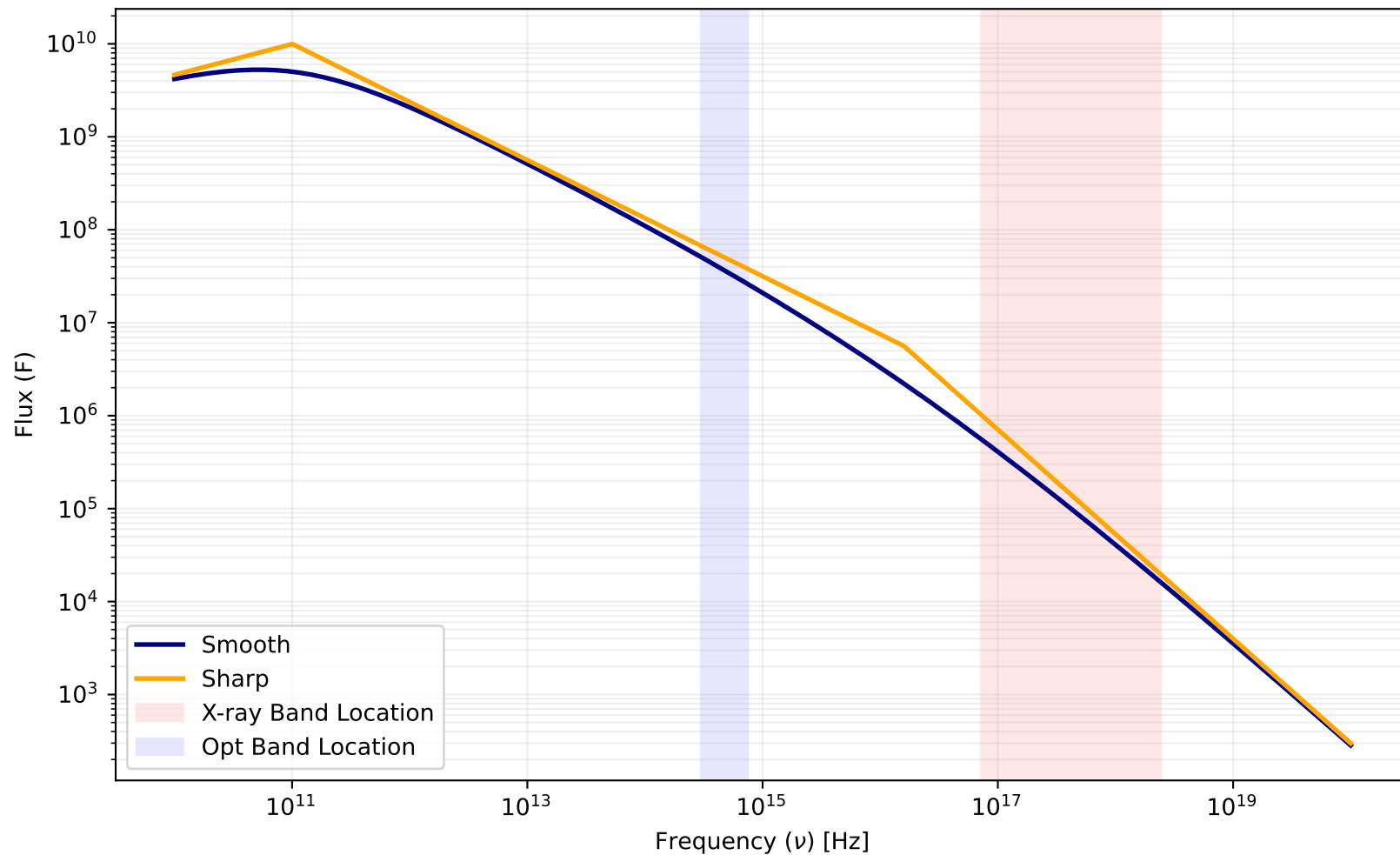
Smooth vs. Sharp Spectral Model ( p = 2.25 , \nu_c = 1.585\text{e}+16 )
