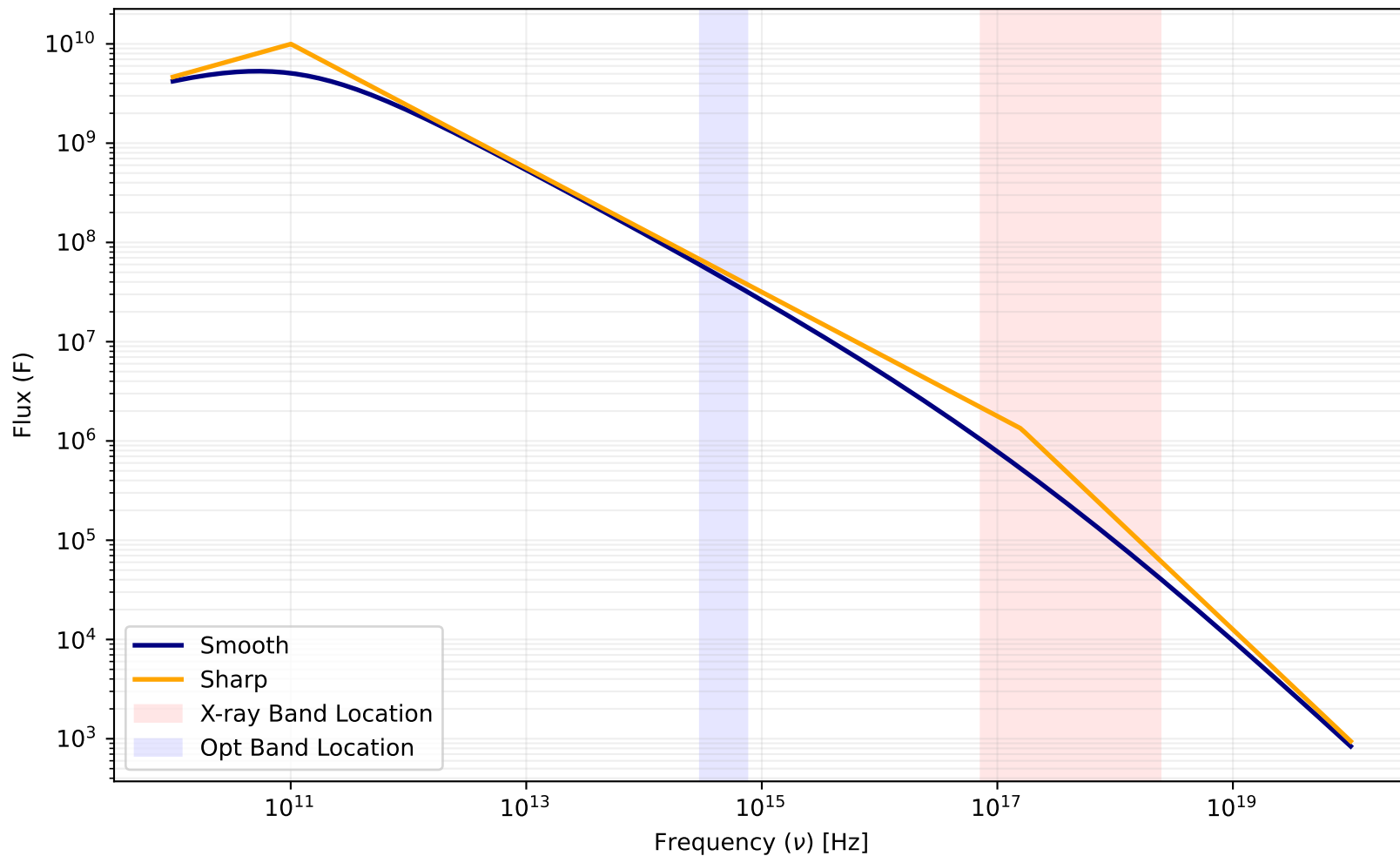
Smooth vs. Sharp Spectral Model ( p = 2.25 , \nu_c = 1.585\text{e}+17 )
