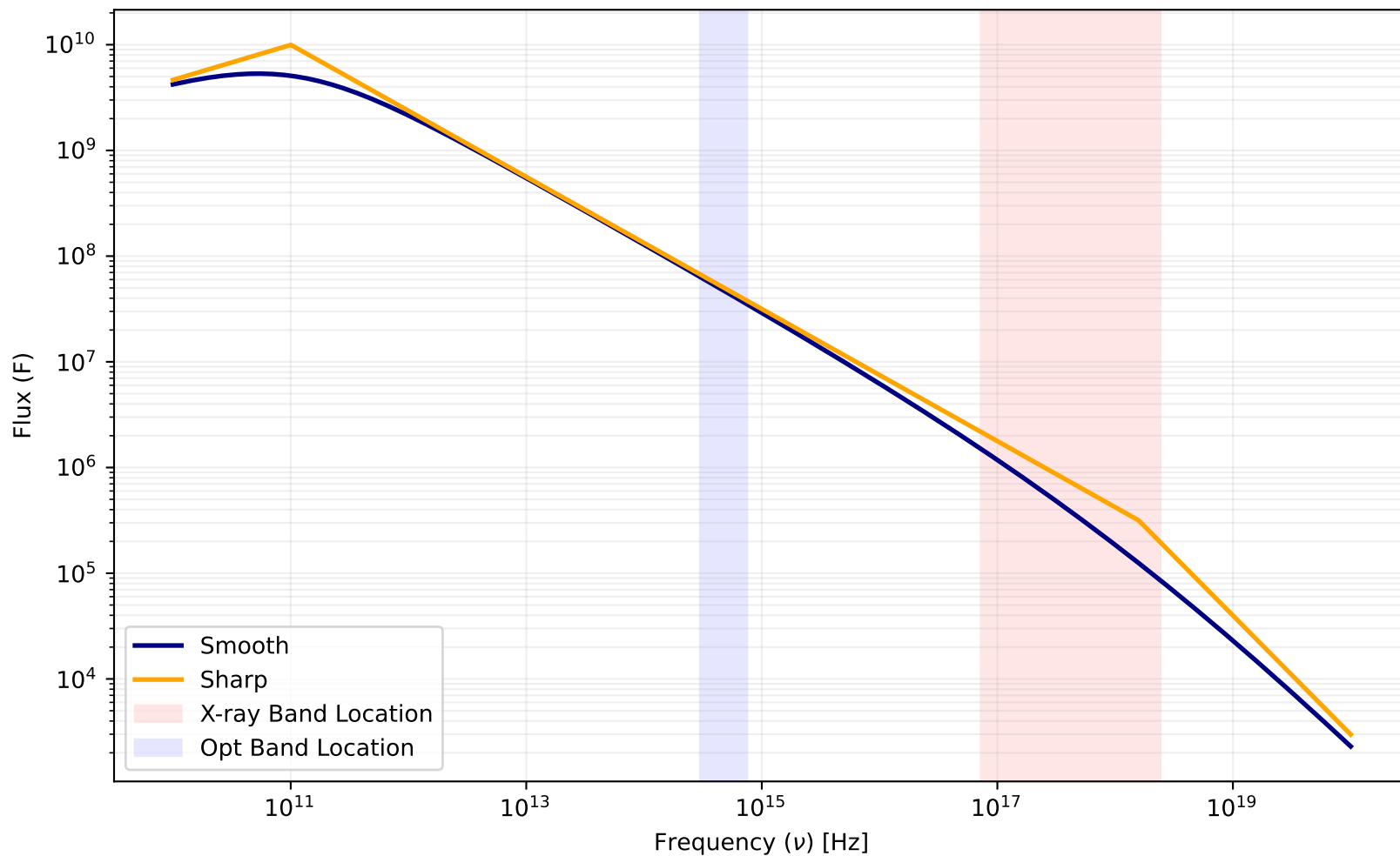
Smooth vs. Sharp Spectral Model ( p = 2.25 , \nu_c = 1.585\text{e}+18 )
