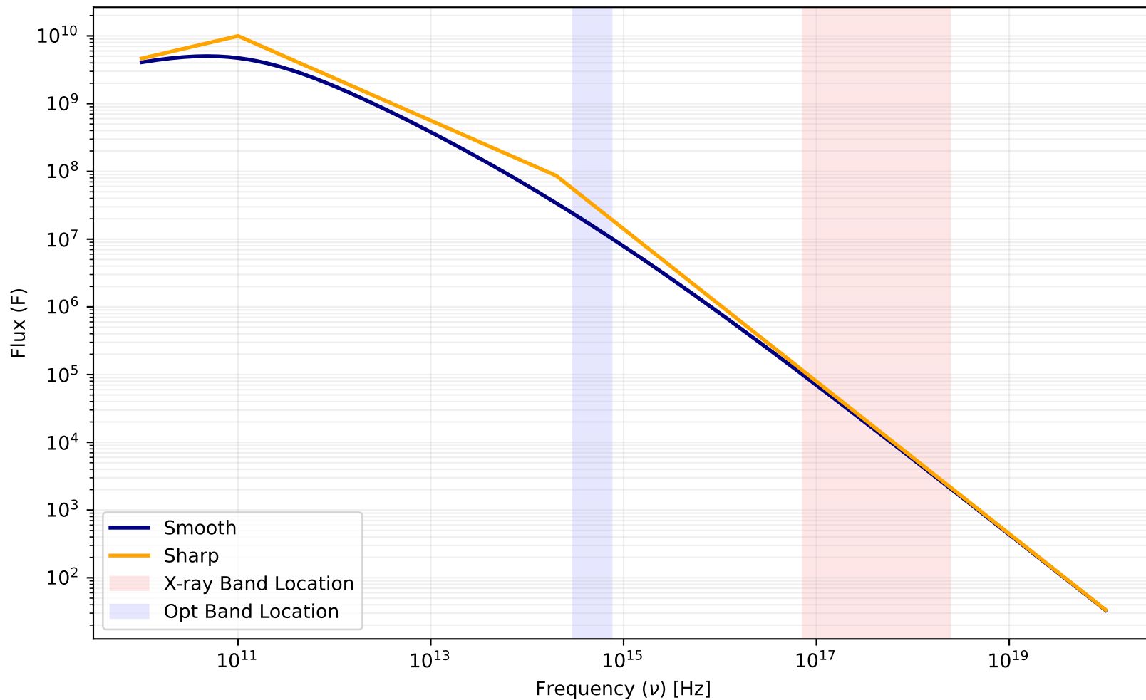
Smooth vs. Sharp Spectral Model ( p = 2.25 , \nu_c = 1.995\text{e}+14 )
