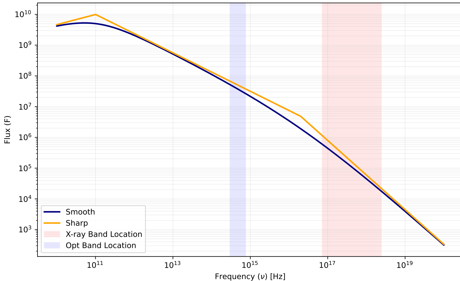
Smooth vs. Sharp Spectral Model ( p = 2.25 , \nu_c = 1.995\text{e}+16 )
