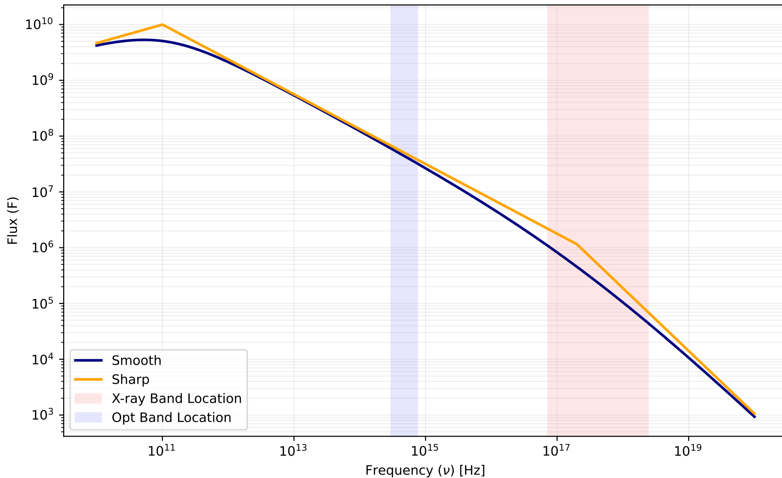
Smooth vs. Sharp Spectral Model ( p = 2.25 , \nu_c = 1.995\text{e}+17 )
