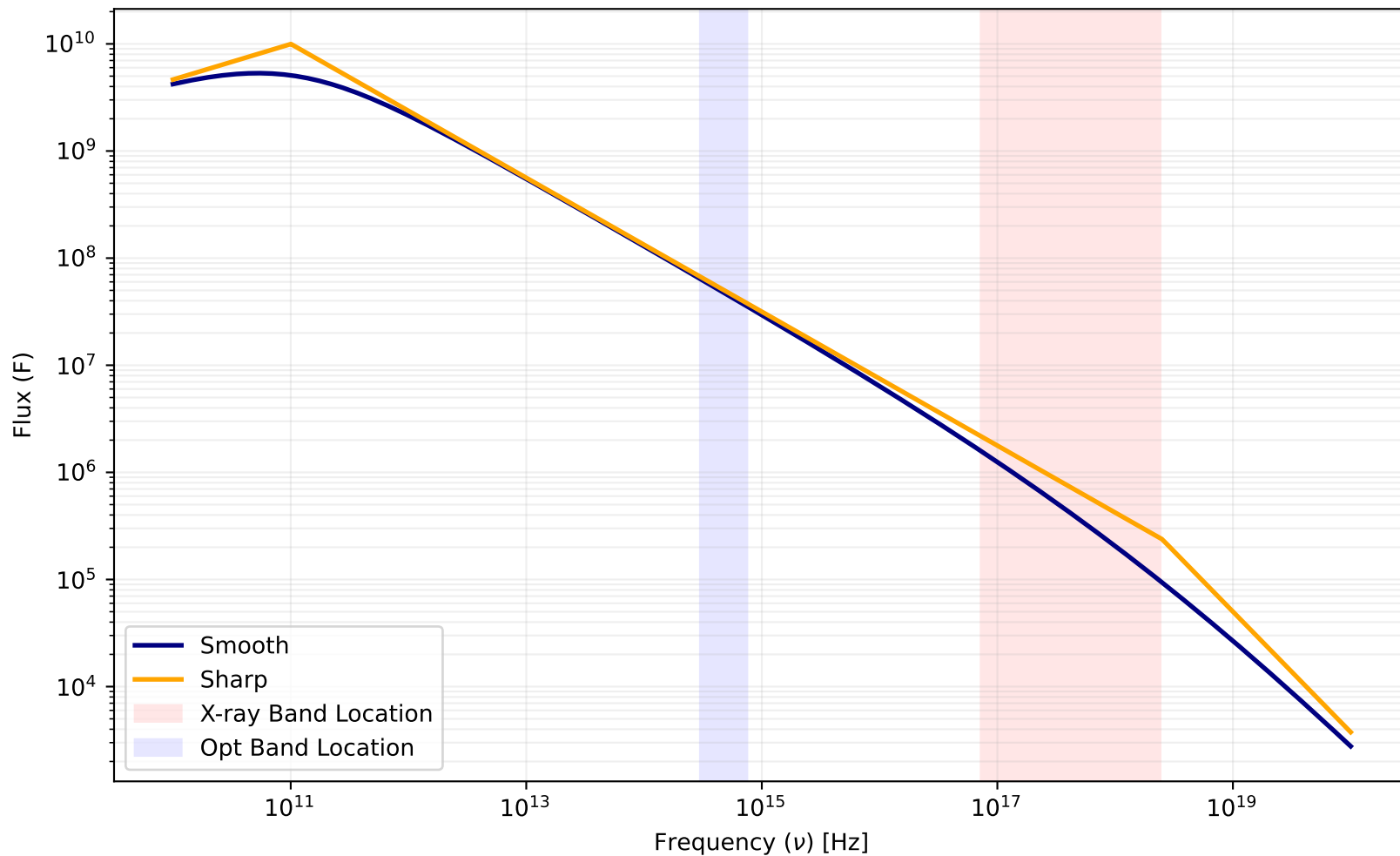
Smooth vs. Sharp Spectral Model ( p = 2.25 , \nu_c = 2.512 \times 10^{18} )
