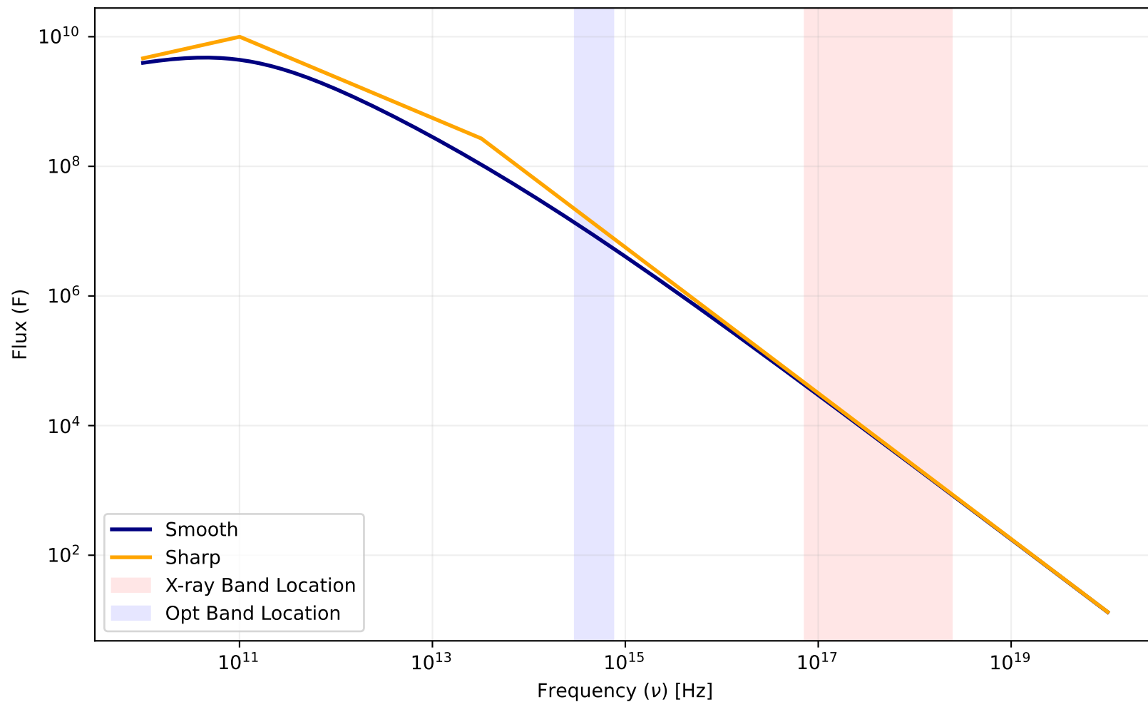
Smooth vs. Sharp Spectral Model ( p = 2.25 , \nu_c = 3.162\text{e}+13 )
