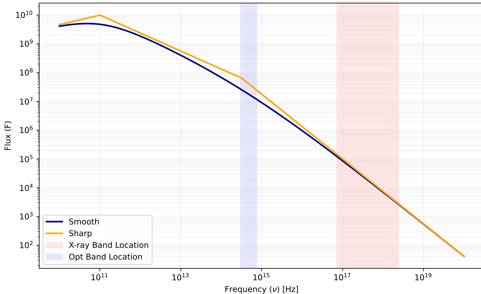
Smooth vs. Sharp Spectral Model ( p = 2.25 , \nu_c = 3.162 \times 10^{14} )
