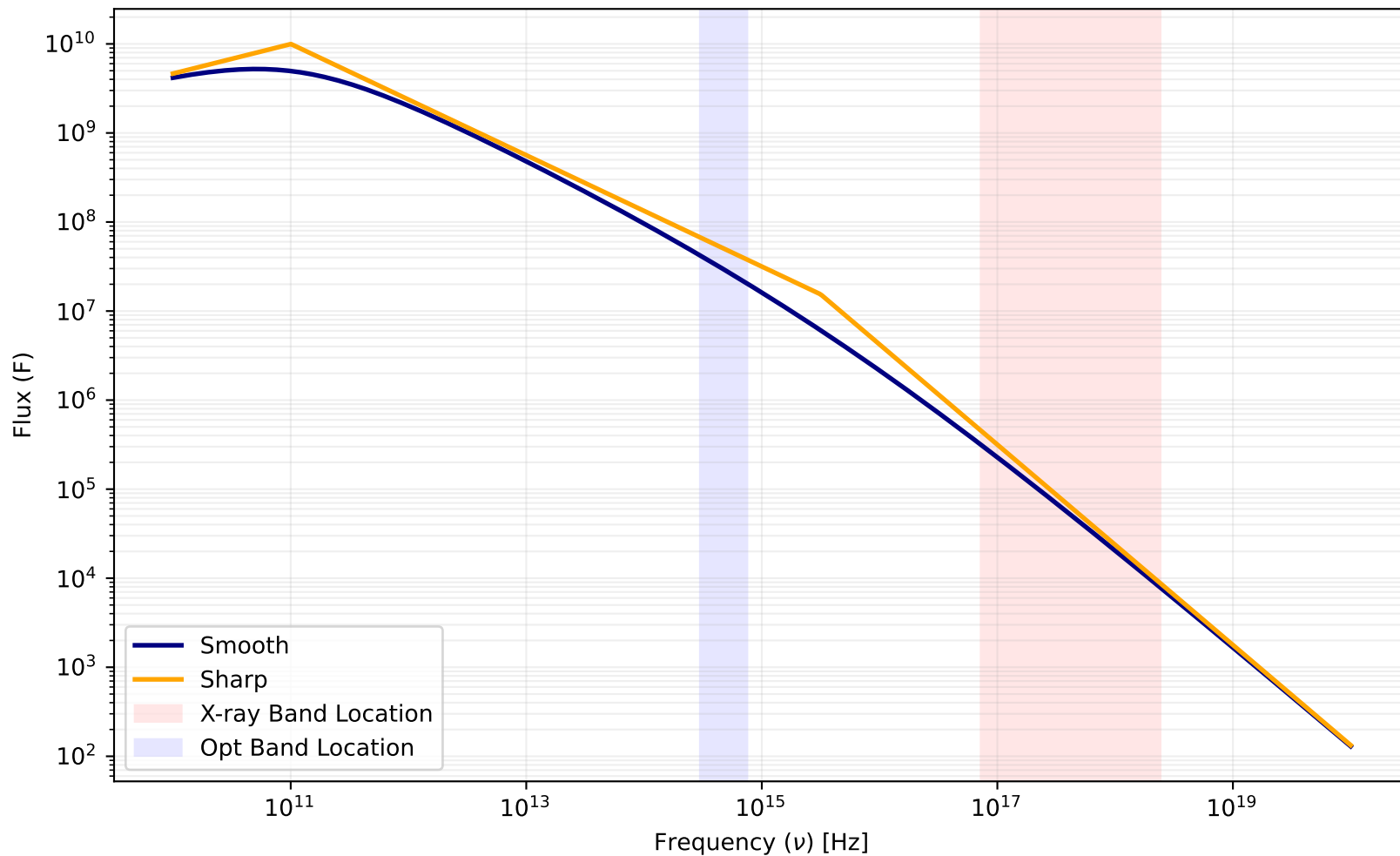
Smooth vs. Sharp Spectral Model ( p = 2.25 , \nu_c = 3.162\text{e}+15 )
