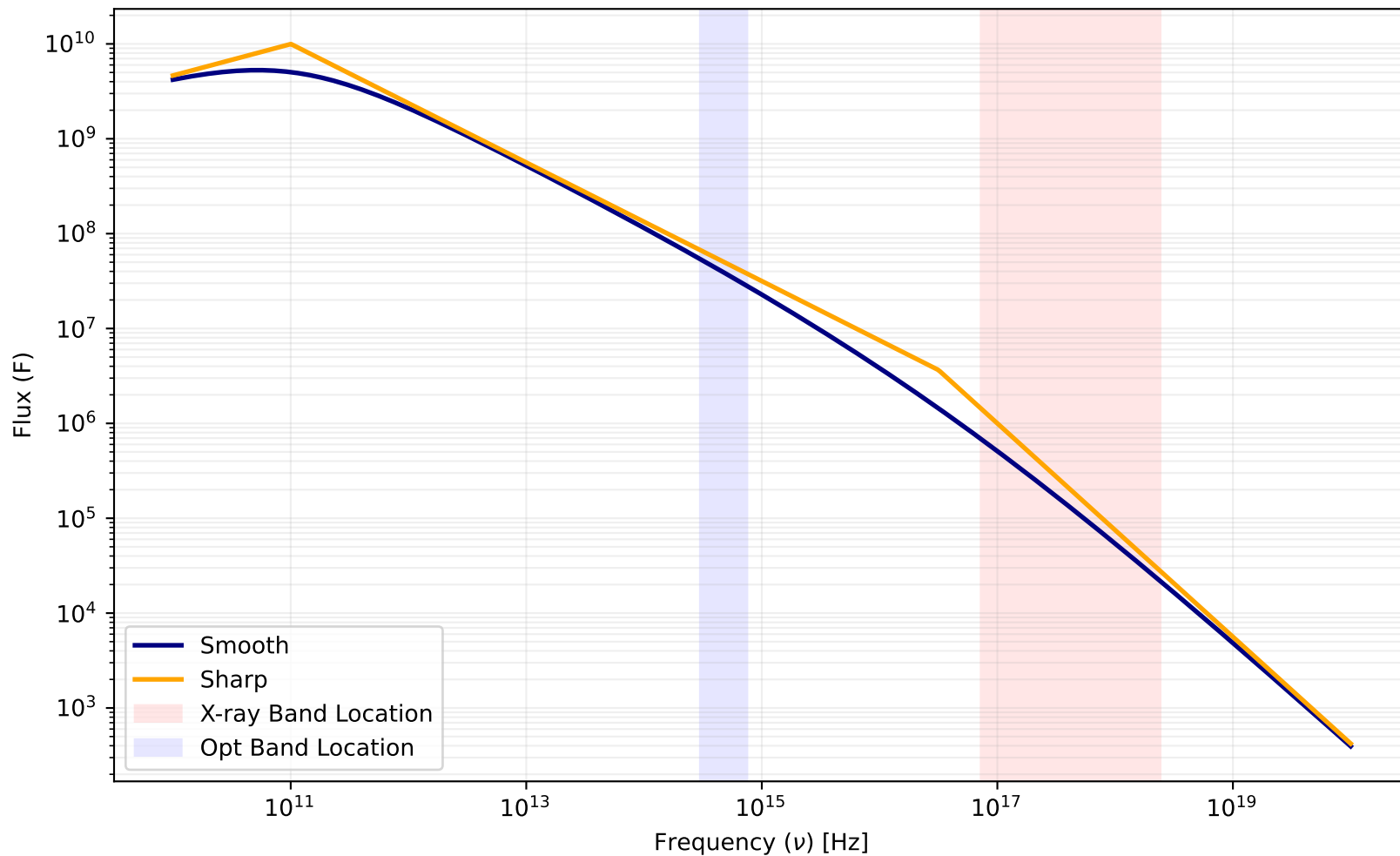
Smooth vs. Sharp Spectral Model ( p = 2.25 , \nu_c = 3.162\text{e}+16 )
