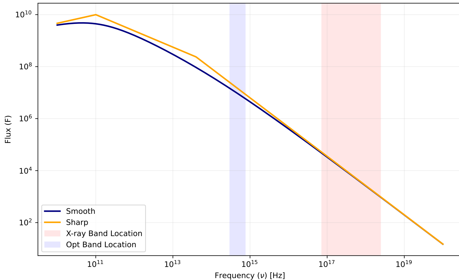
Smooth vs. Sharp Spectral Model ( p = 2.25 , \nu_c = 3.981\text{e}+13 )
