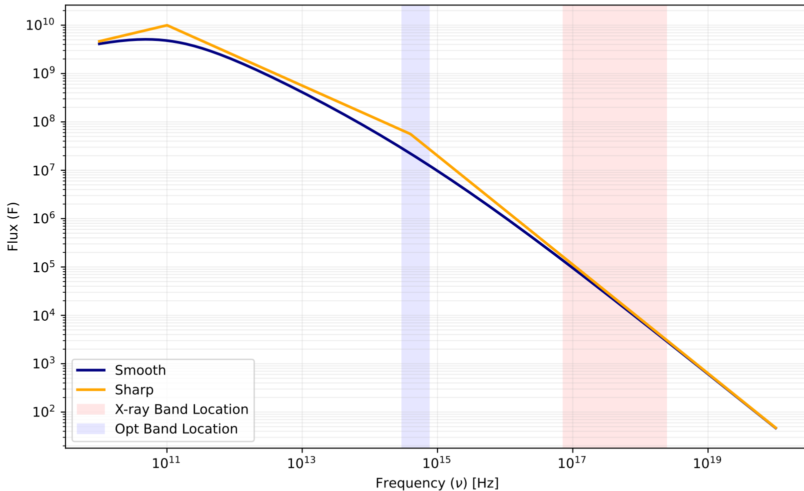
Smooth vs. Sharp Spectral Model ( p = 2.25 , \nu_c = 3.981\text{e}+14 )
