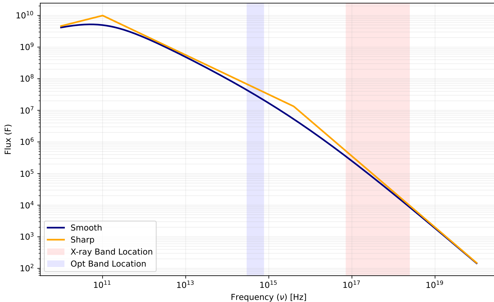
Smooth vs. Sharp Spectral Model ( p = 2.25 , \nu_c = 3.981\text{e}+15 )
