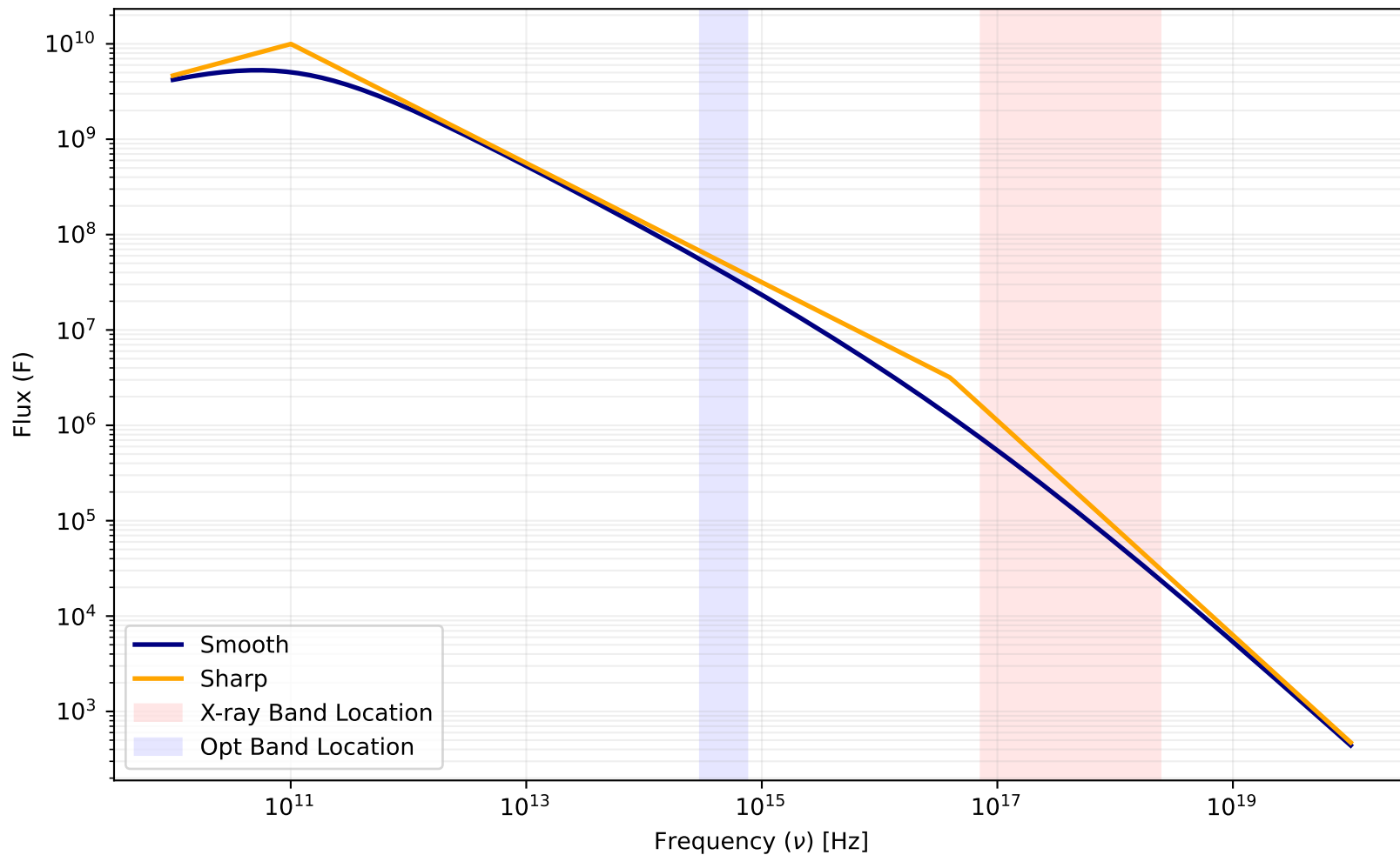
Smooth vs. Sharp Spectral Model ( p = 2.25 , \nu_c = 3.981\text{e}+16 )
