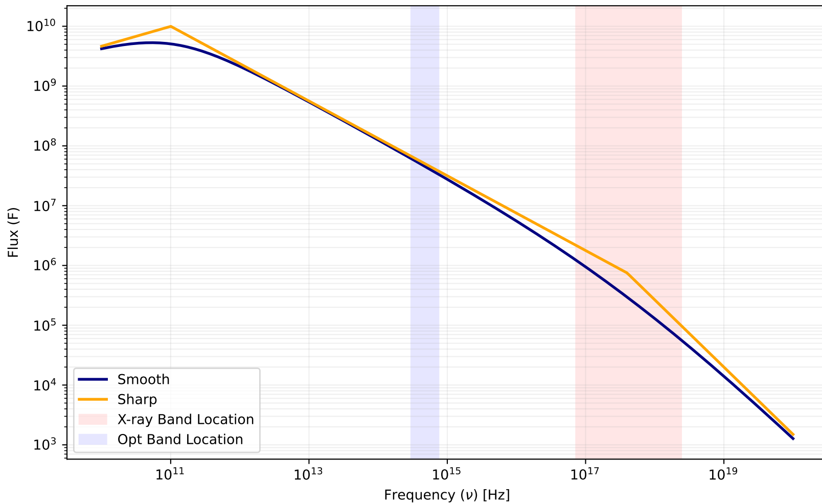
Smooth vs. Sharp Spectral Model ( p = 2.25 , \nu_c = 3.981\text{e}+17 )
