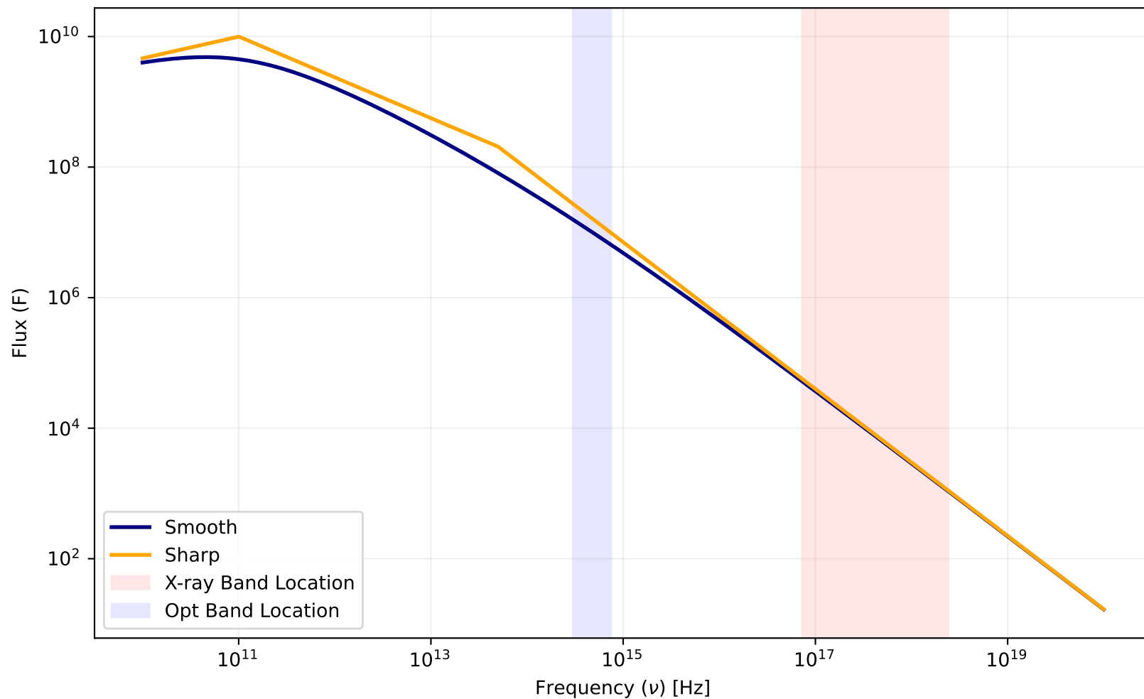
Smooth vs. Sharp Spectral Model ( p = 2.25 , \nu_c = 5.012\text{e}+13 )
