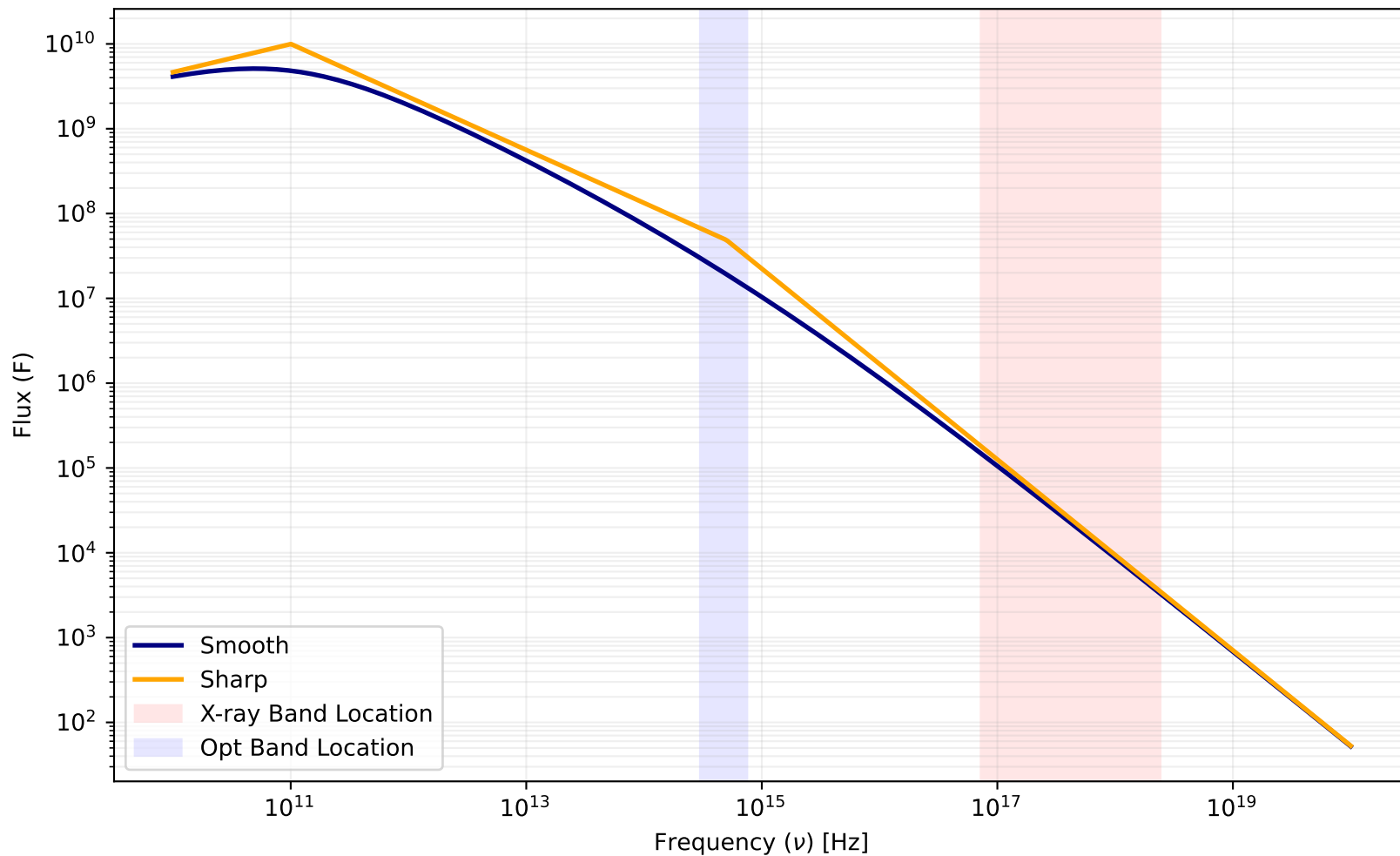
Smooth vs. Sharp Spectral Model ( p = 2.25 , \nu_c = 5.012\text{e}+14 )
