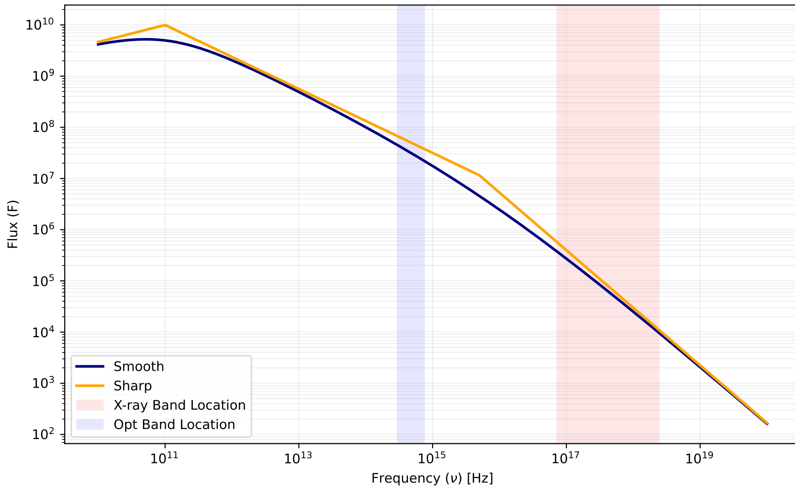
Smooth vs. Sharp Spectral Model ( p = 2.25 , \nu_c = 5.012\text{e}+15 )
