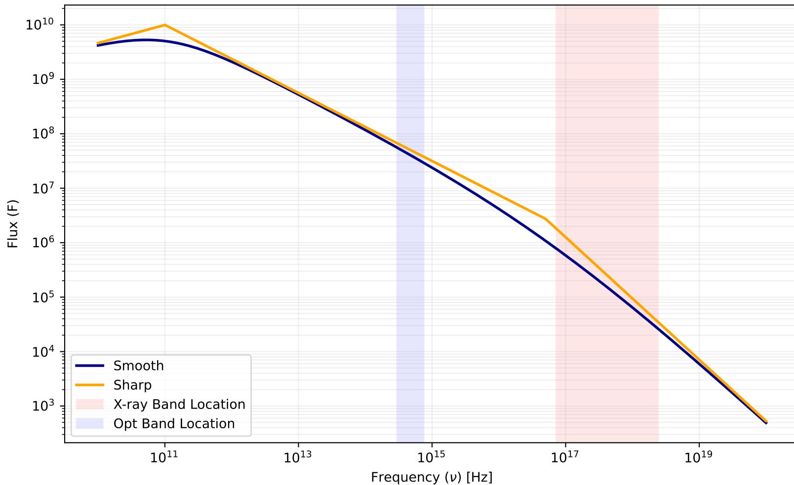
Smooth vs. Sharp Spectral Model ( p = 2.25 , \nu_c = 5.012 \times 10^{16} )
