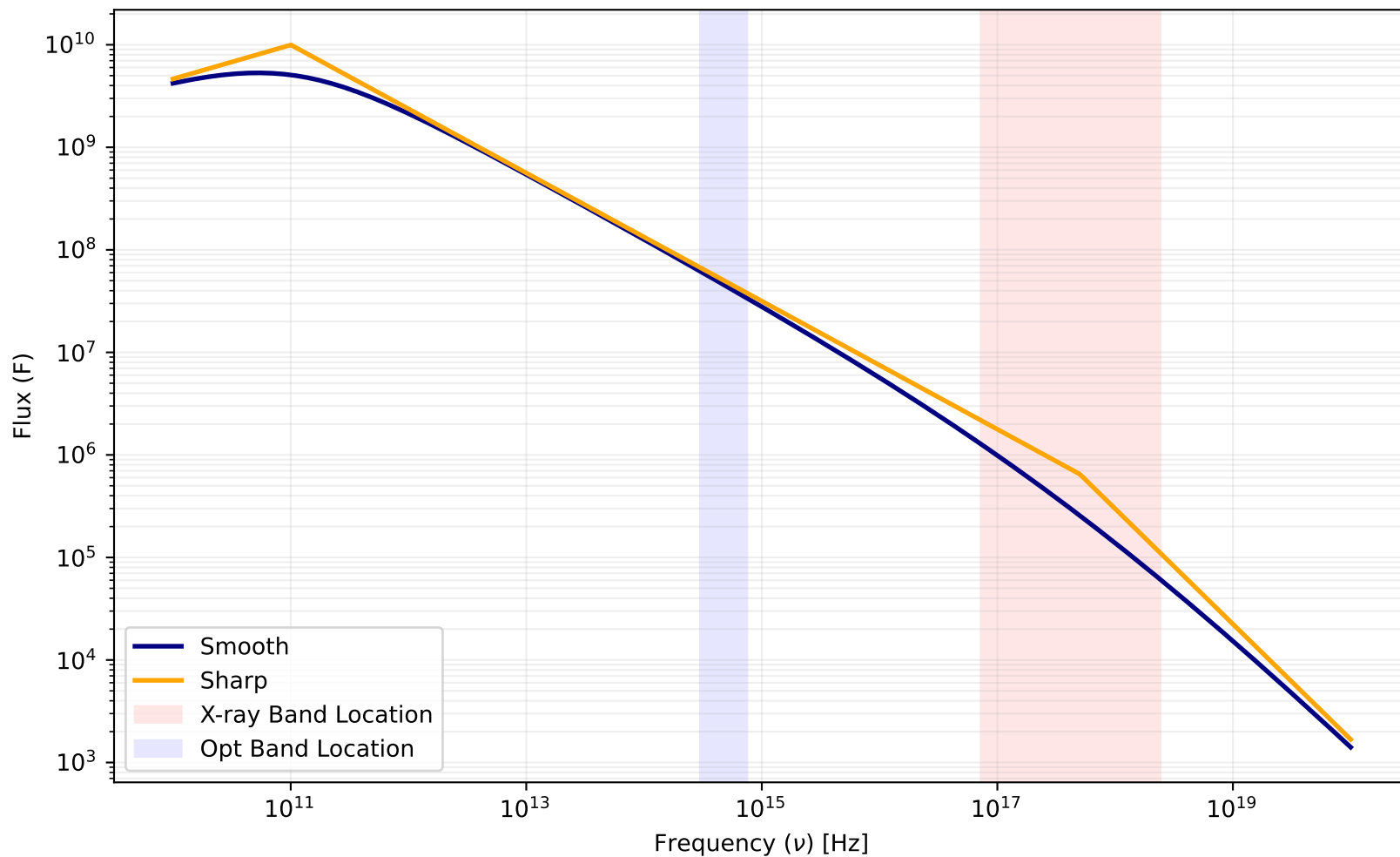
Smooth vs. Sharp Spectral Model ( p = 2.25 , \nu_c = 5.012\text{e}+17 )
