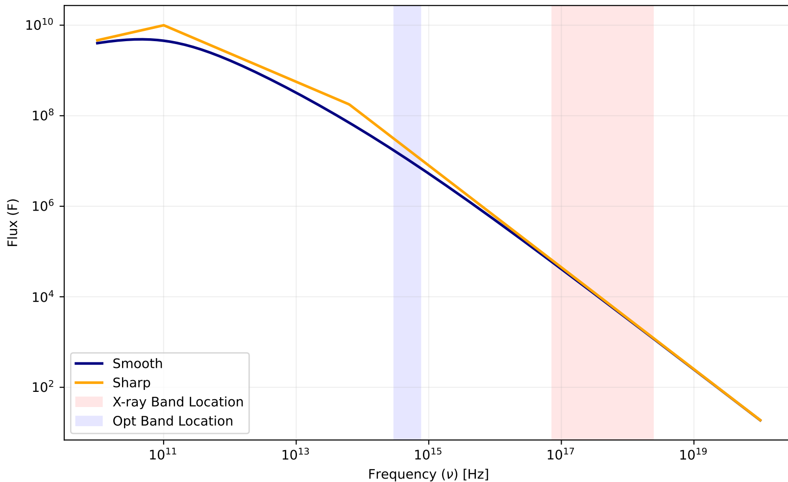
Smooth vs. Sharp Spectral Model ( p = 2.25 , \nu_c = 6.310\text{e}+13 )
