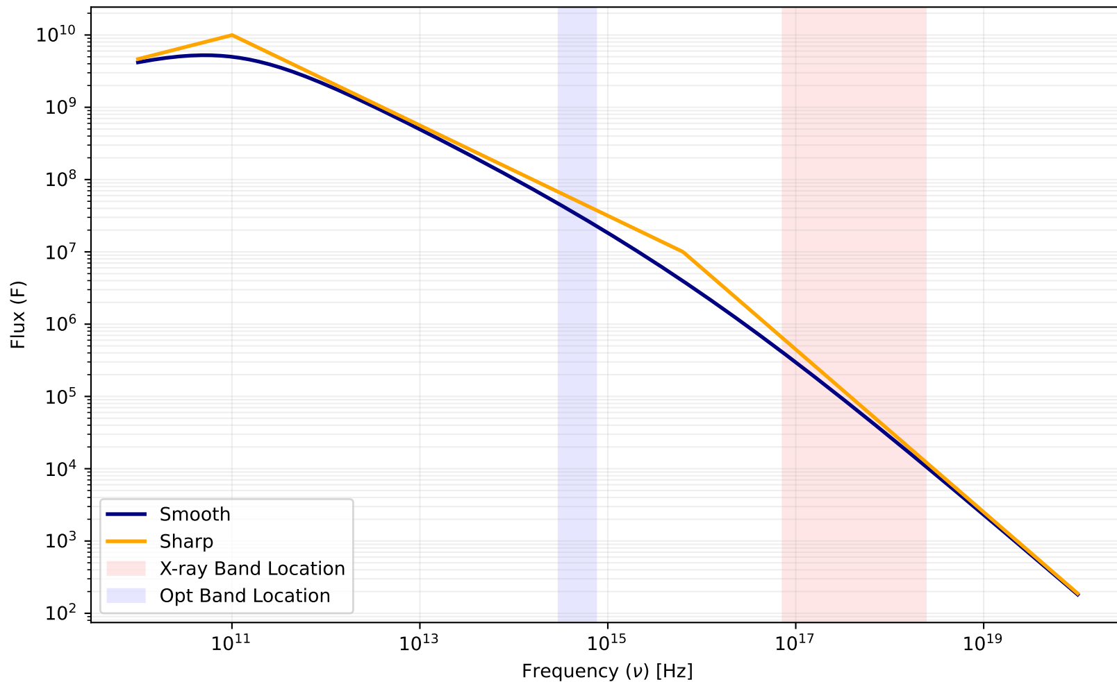
Smooth vs. Sharp Spectral Model ( p = 2.25 , \nu_c = 6.310\text{e}+15 )
