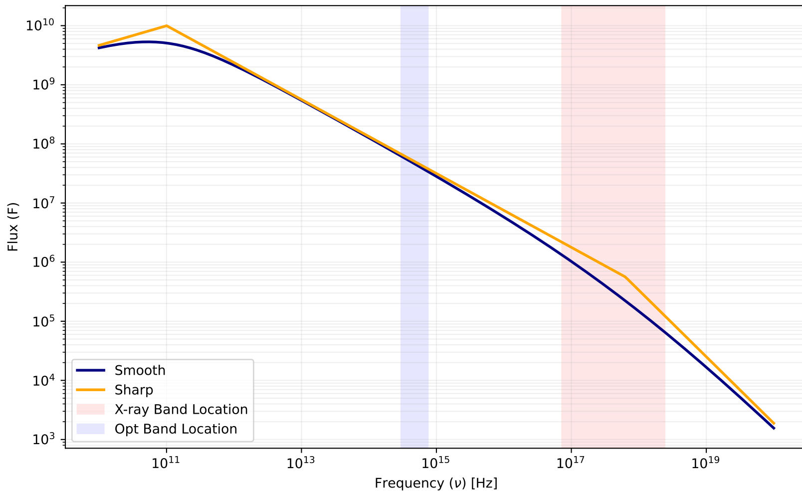
Smooth vs. Sharp Spectral Model ( p = 2.25 , \nu_c = 6.310\text{e}+17 )
