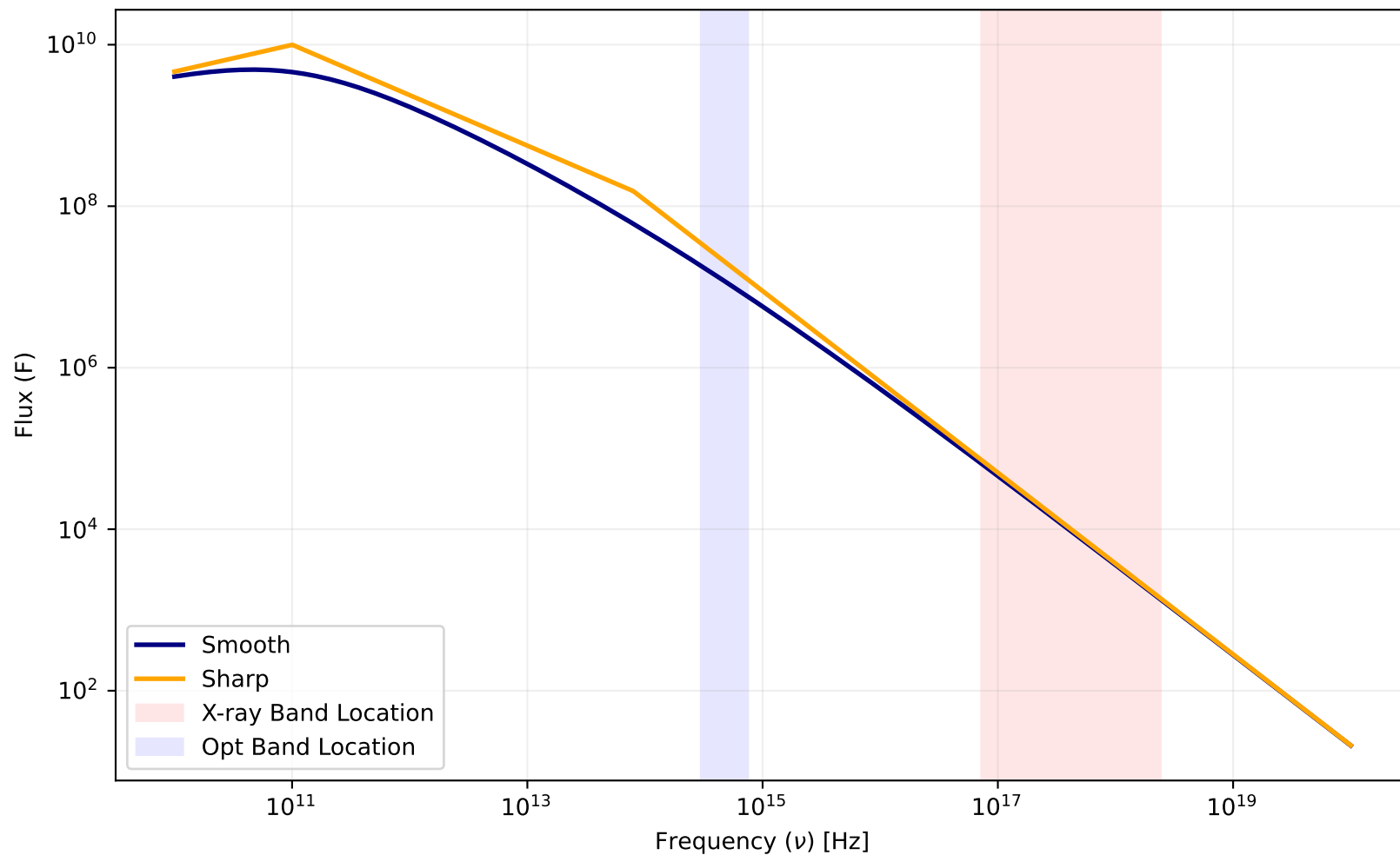
Smooth vs. Sharp Spectral Model ( p = 2.25 , \nu_c = 7.943\text{e}+13 )
