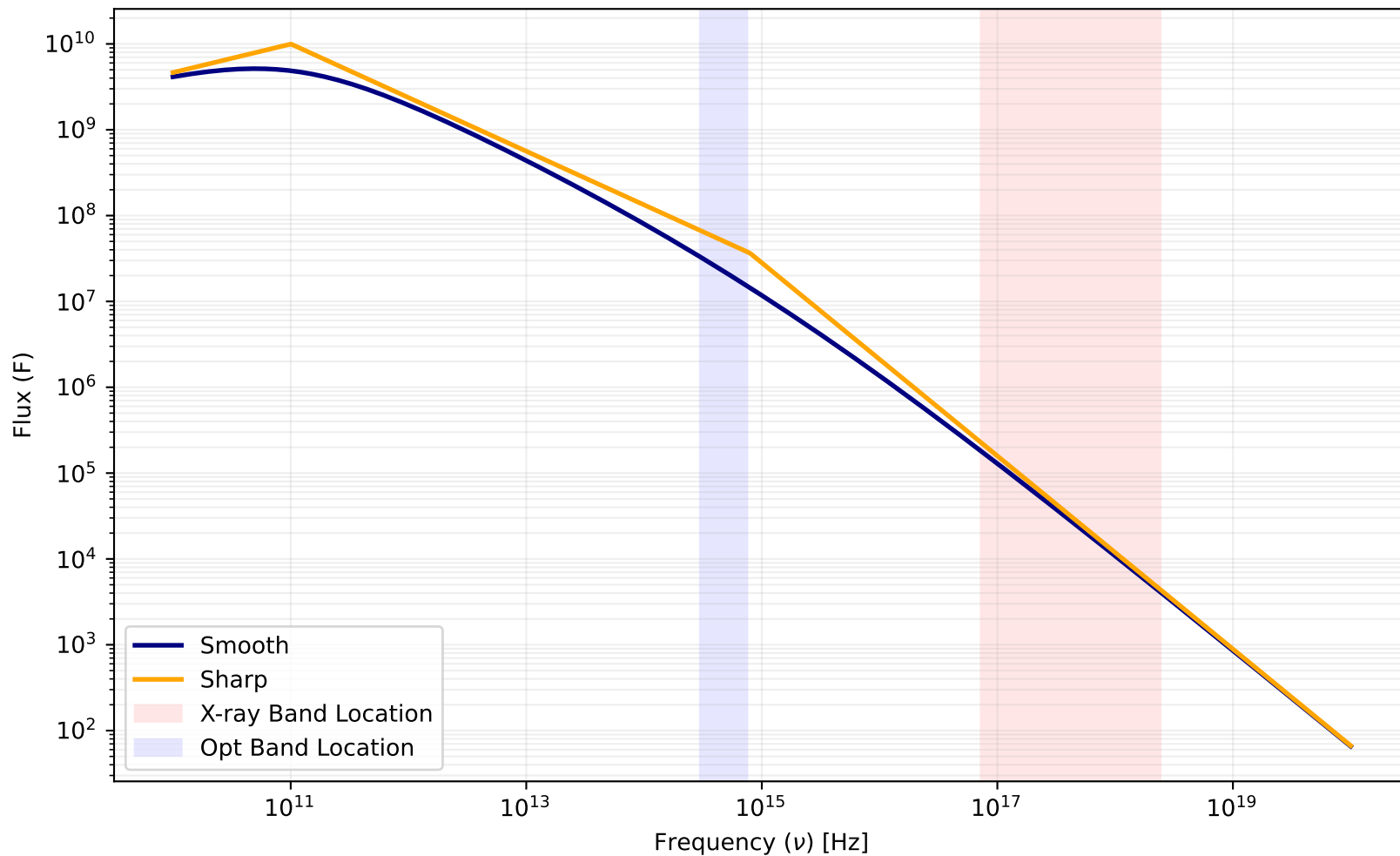
Smooth vs. Sharp Spectral Model ( p = 2.25 , \nu_c = 7.943\text{e}+14 )
