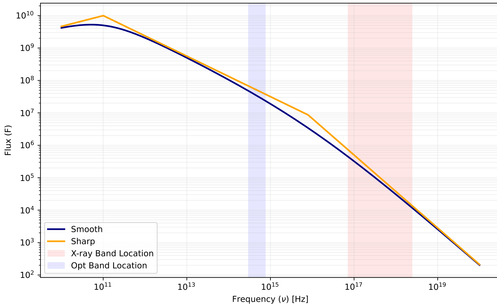
Smooth vs. Sharp Spectral Model ( p = 2.25 , \nu_c = 7.943\text{e}+15 )
