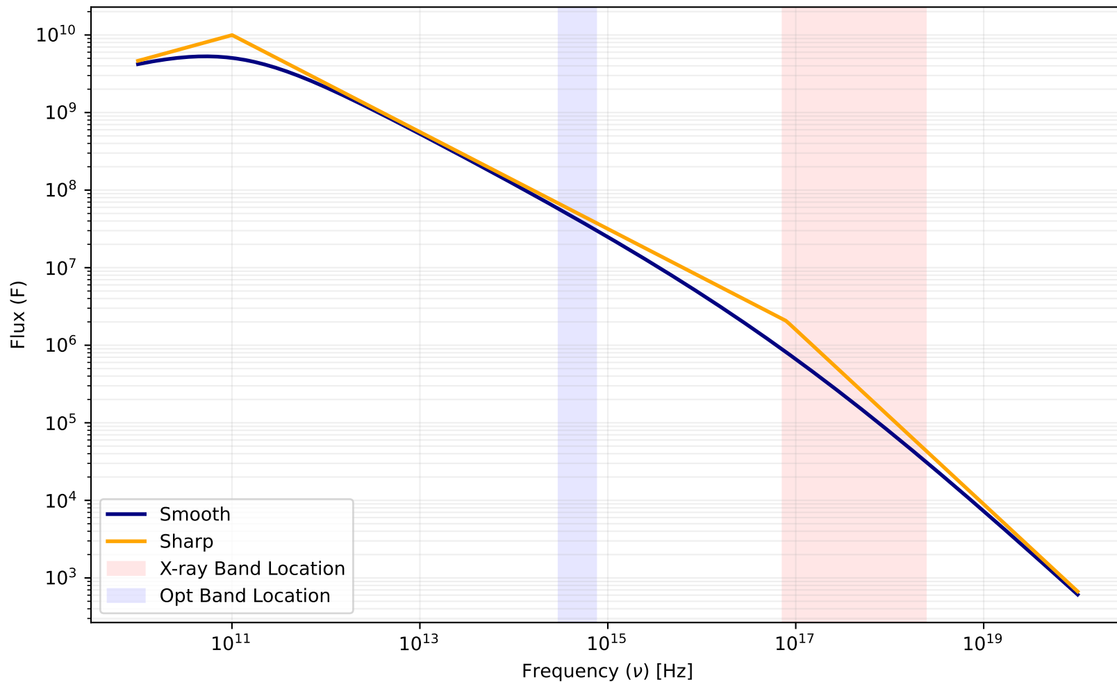
Smooth vs. Sharp Spectral Model ( p = 2.25 , \nu_c = 7.943\text{e}+16 )
