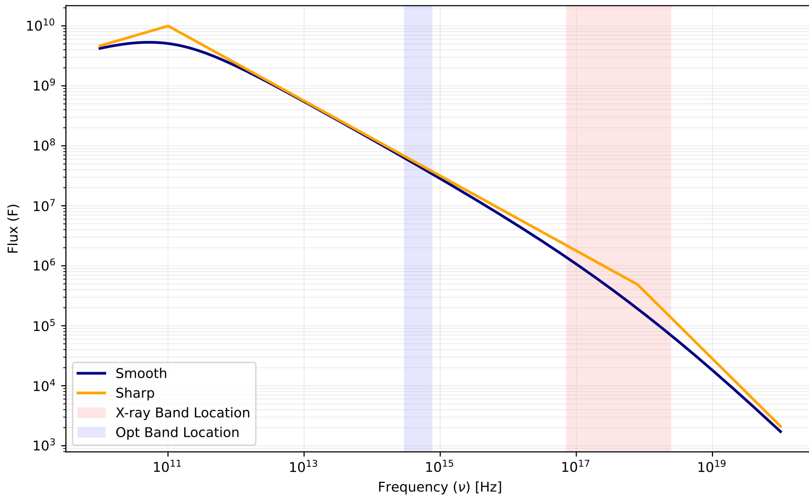
Smooth vs. Sharp Spectral Model ( p = 2.25 , \nu_c = 7.943\text{e}+17 )
