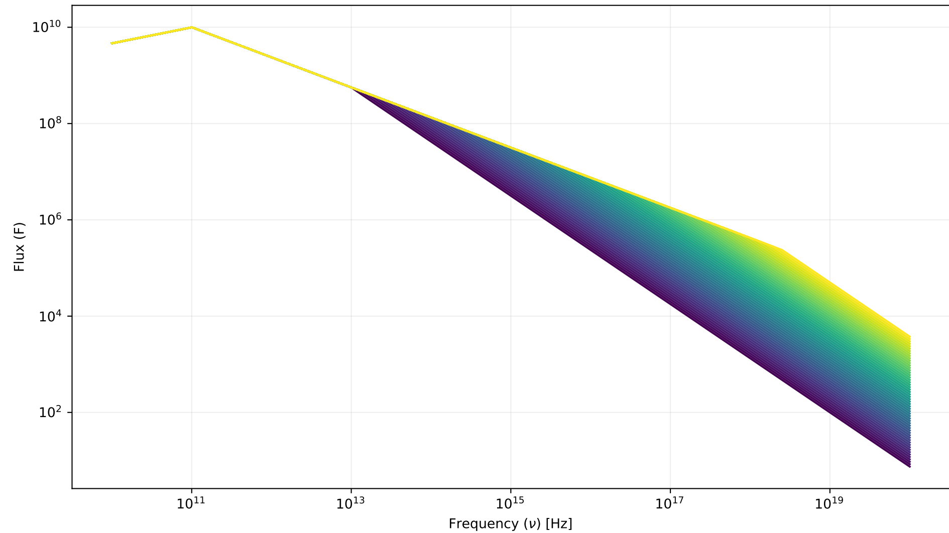
Sharp Spectral Model for Changing \nu_c ( p = 2.25 )
