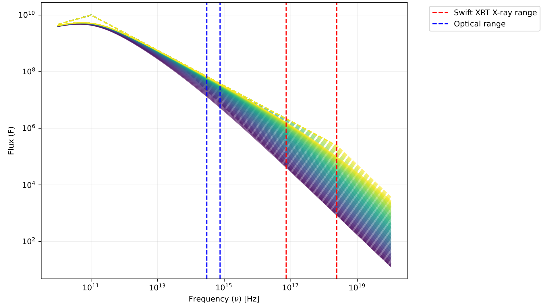
Smooth vs. Sharp Spectral Models for Changing \nu_c ( p = 2.25 )
