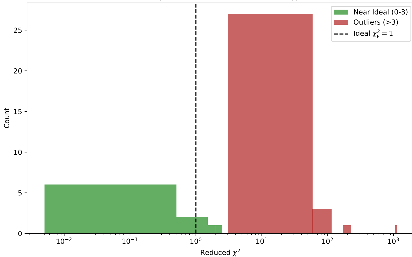
Categorized Distribution of Reduced \chi^2
