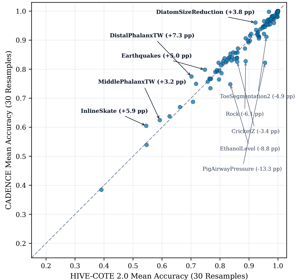
(b) CADENCE vs. HIVE-COTE 2.0 (39 Wins / 7 Ties / 63 Losses, Mean Diff: -0.32 pp, p = 0.295 )
