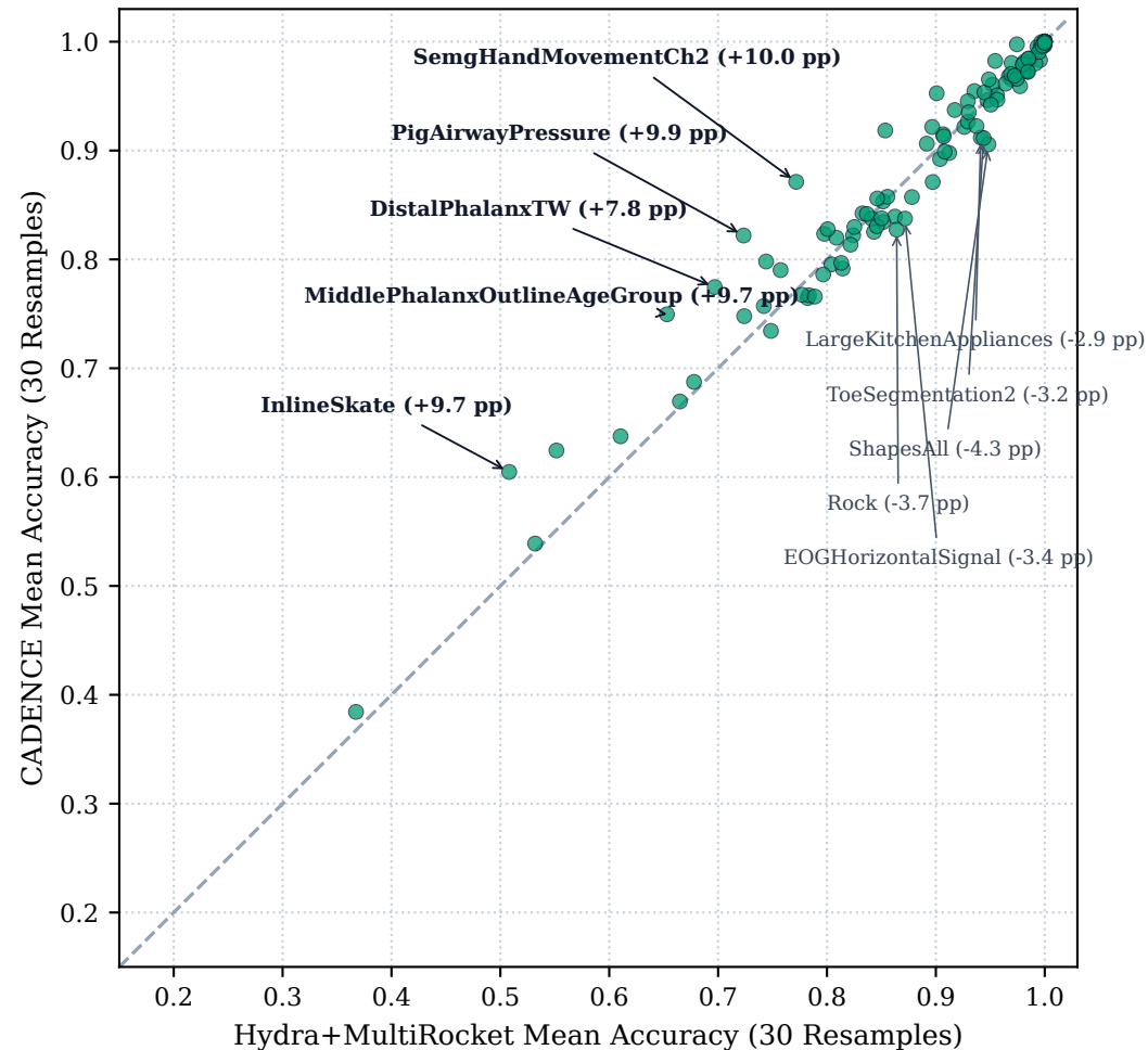
(a) CADENCE vs. Hydra+MultiRocket (46 Wins / 7 Ties / 56 Losses, Mean Gain: +0.46 pp)
