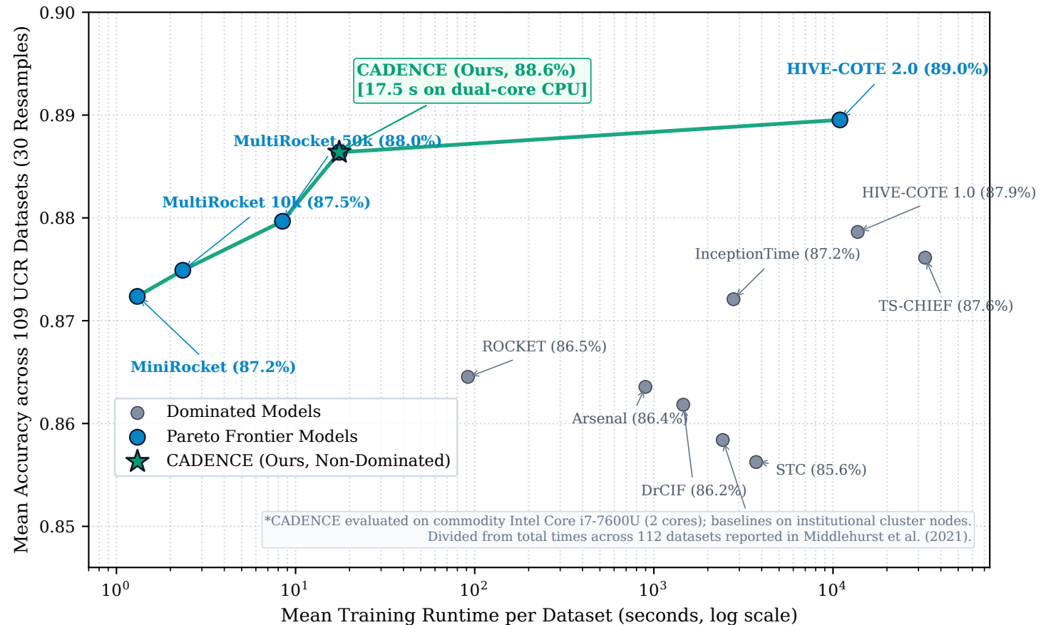
Empirical Pareto Frontier: Accuracy vs. Training Runtime
