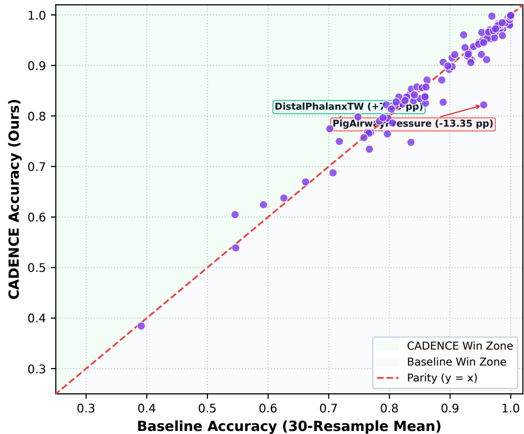
CADENCE vs HIVE-COTE 2.0 (Wins: 39 | Ties: 7 | Losses: 63)
