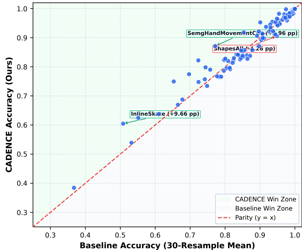
CADENCE vs Hydra+MultiRocket (Wins: 46 | Ties: 7 | Losses: 56)
