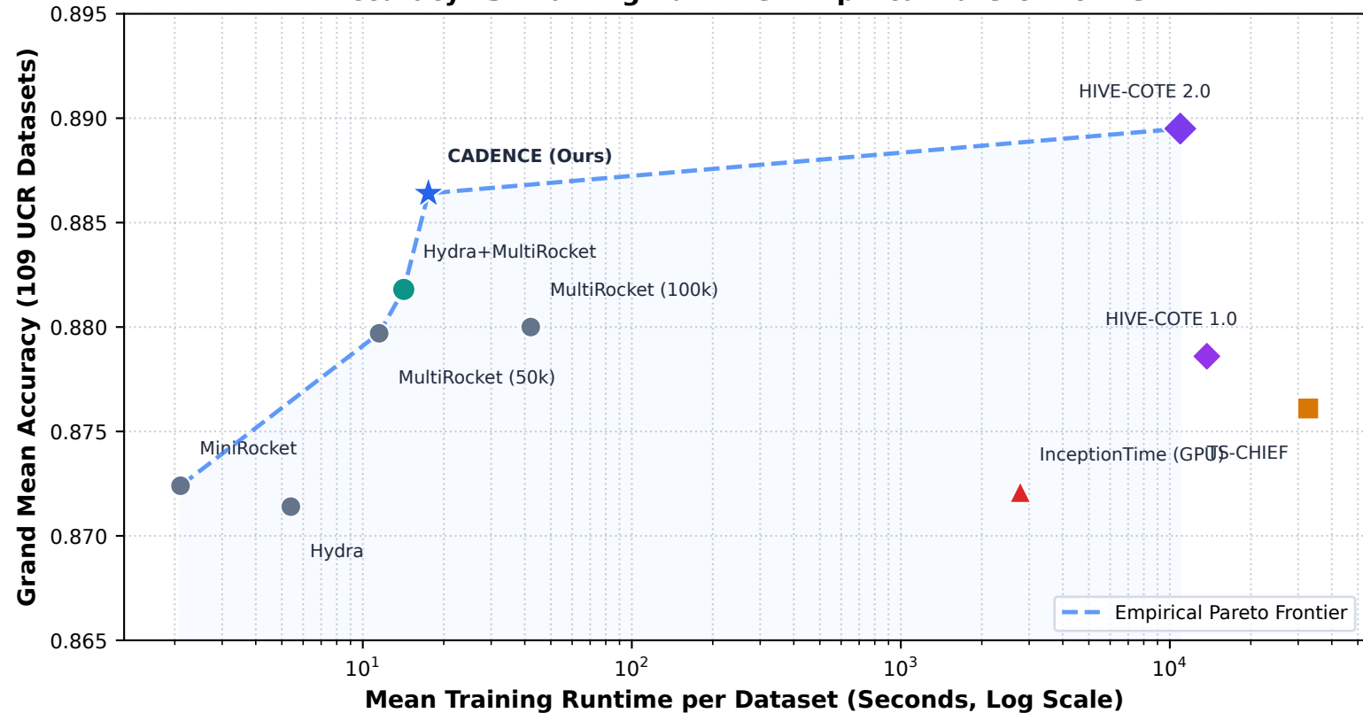
Accuracy vs. Training Runtime: Empirical Pareto Frontier
