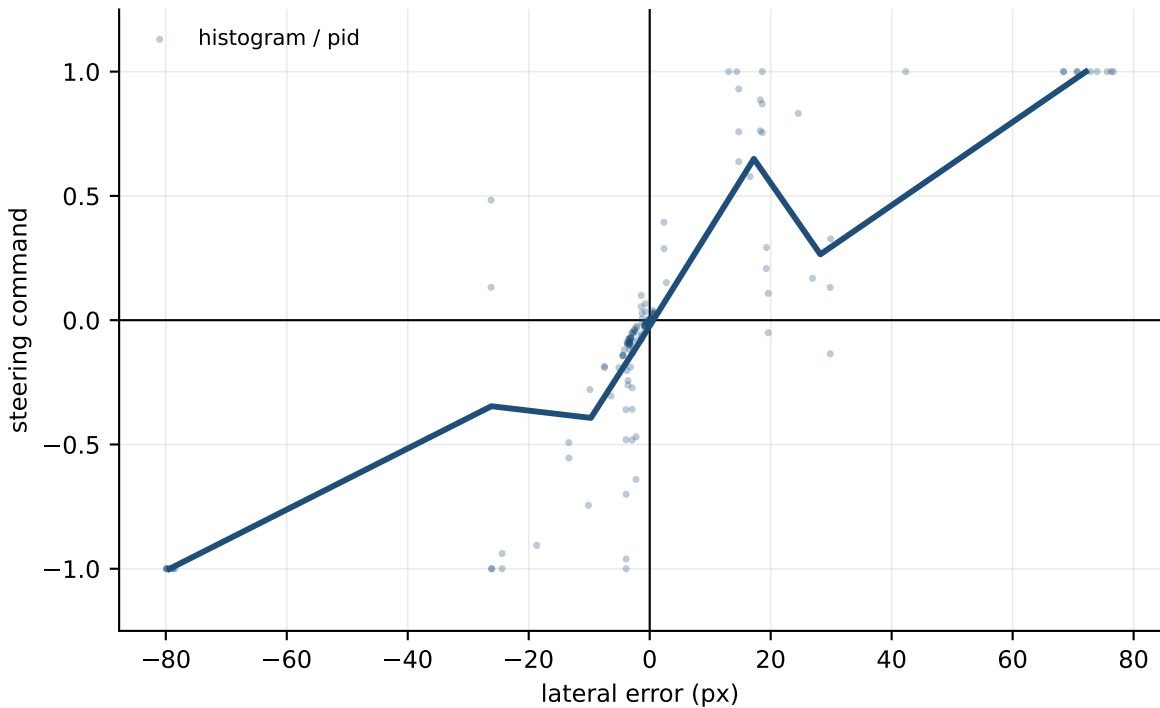
Controller characteristic: commanded steering against measured error
