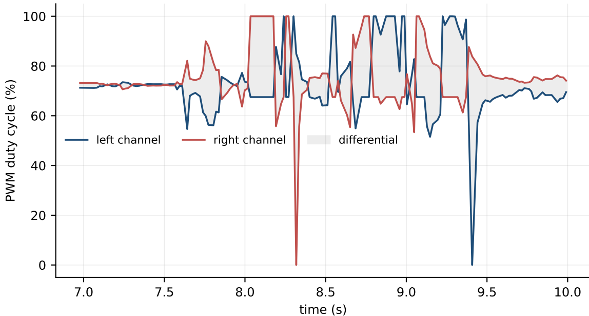
Motor duty cycles (PID)
