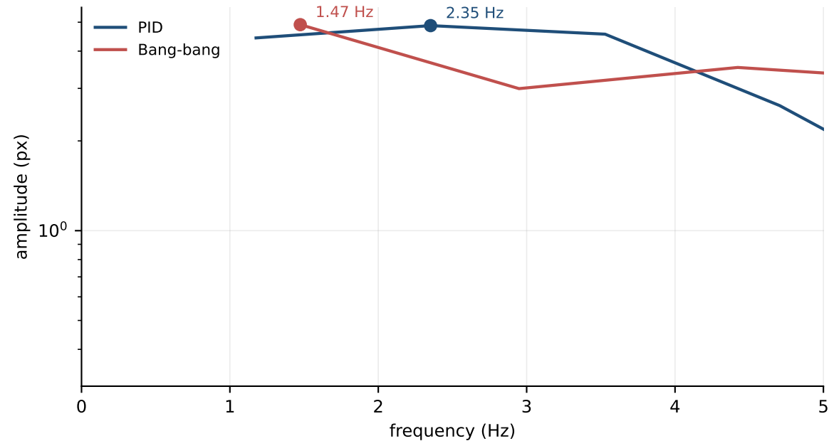
Averaged power spectrum of the lateral error
