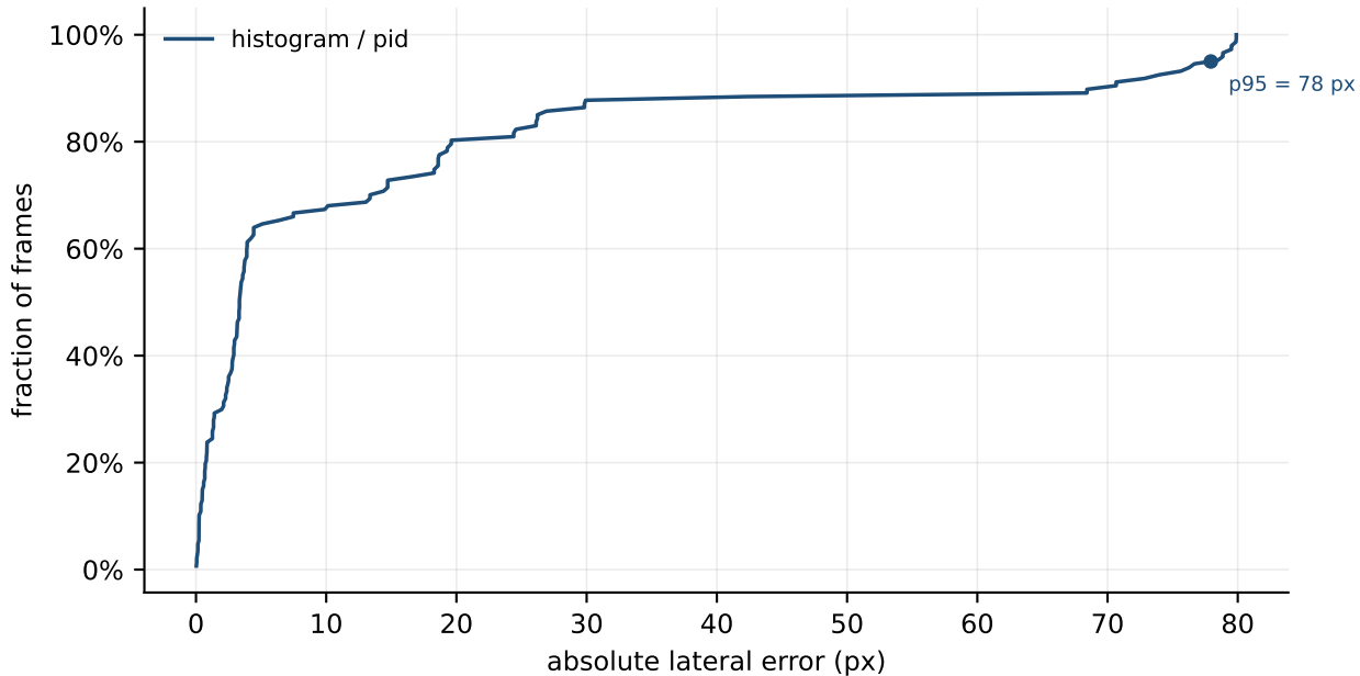
Cumulative distribution of the absolute lateral error
