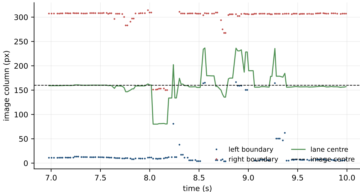
Detected lane boundaries (histogram / pid)
