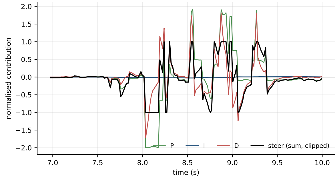
PID term contributions (PID)
