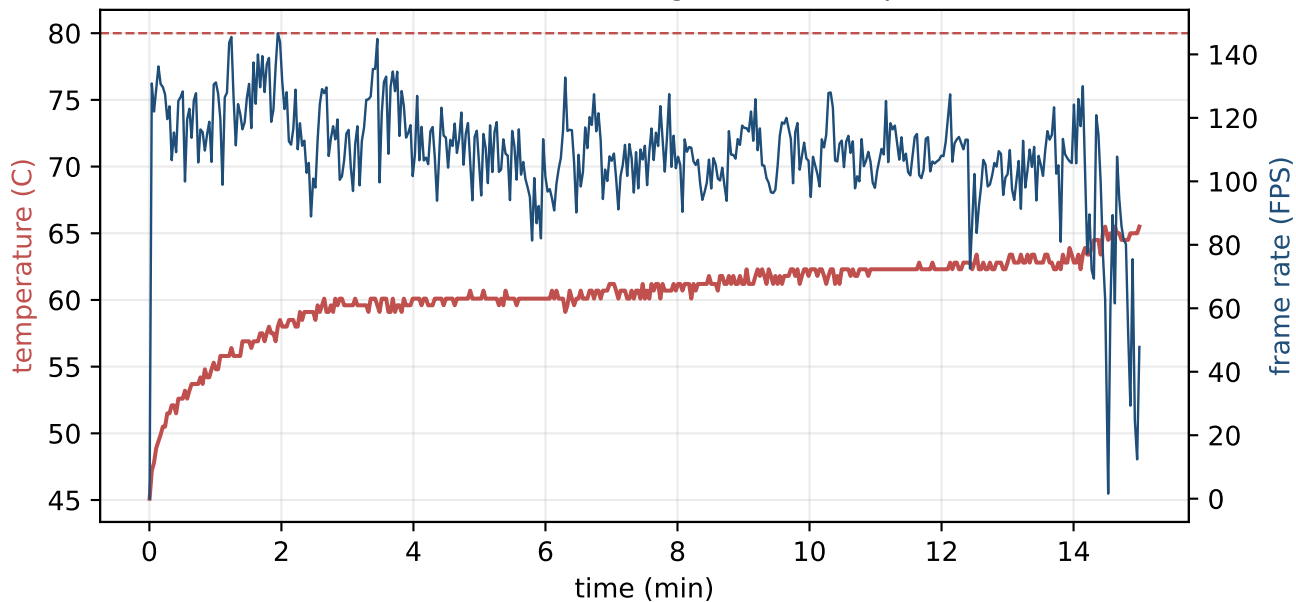
Thermal behaviour during sustained operation
