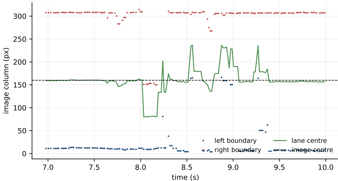
Detected lane boundaries (Histogram)
