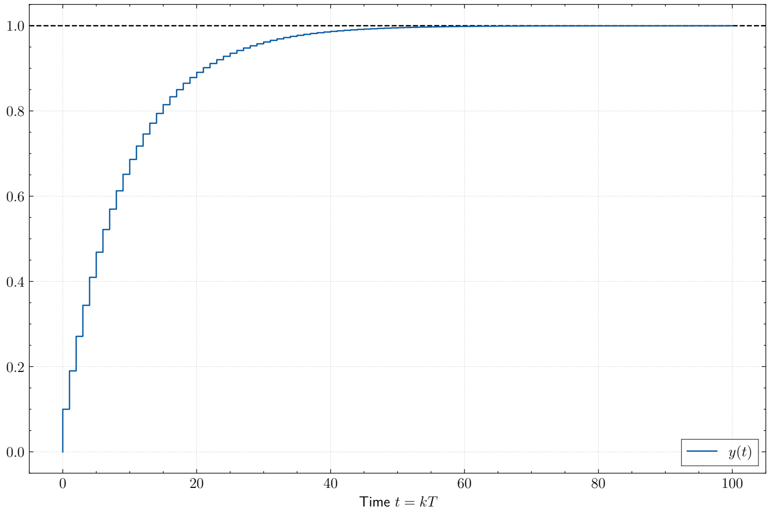
Step response
