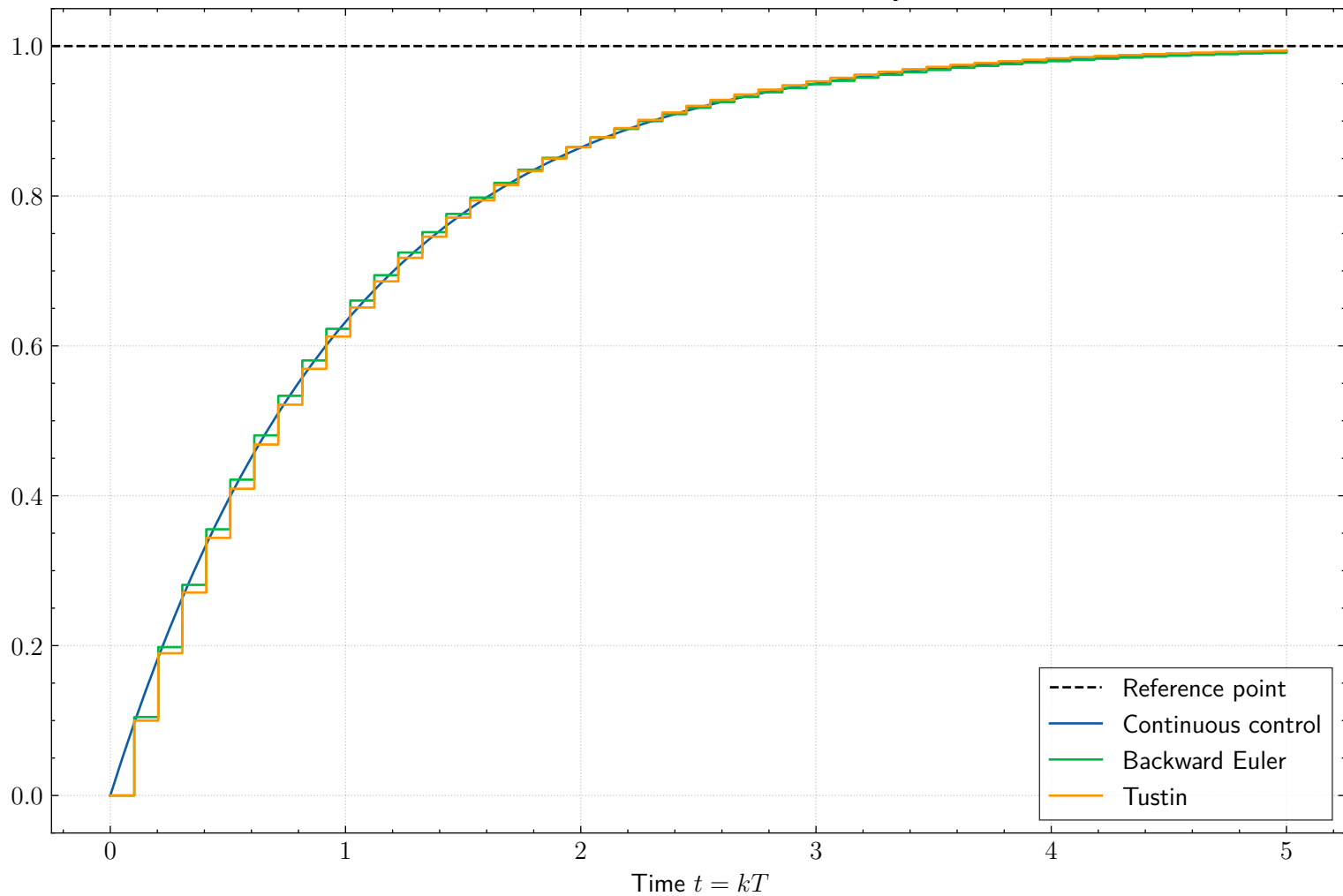
Discretized PI control of first-order system
