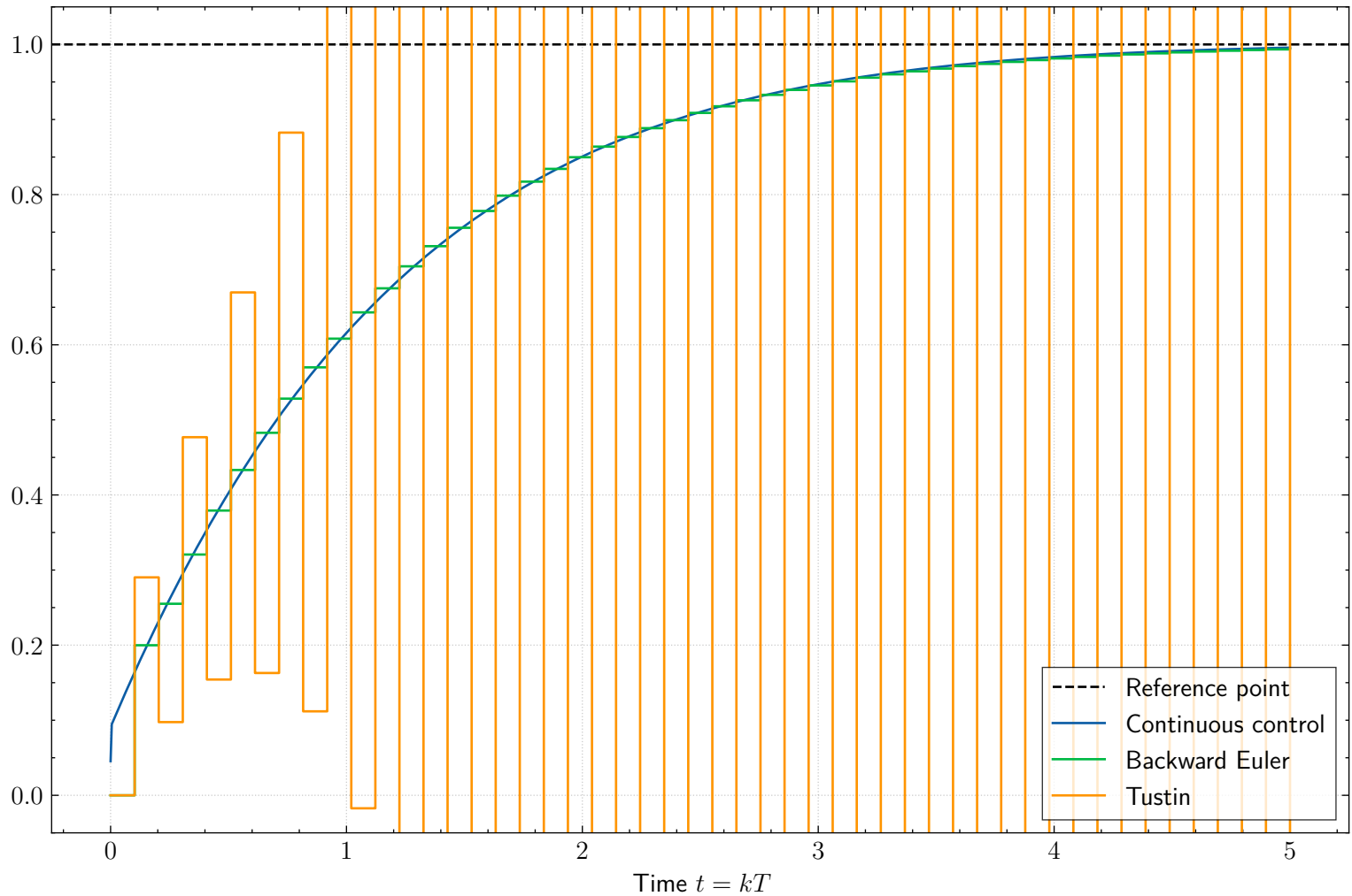
Discretized PID control of first-order system
