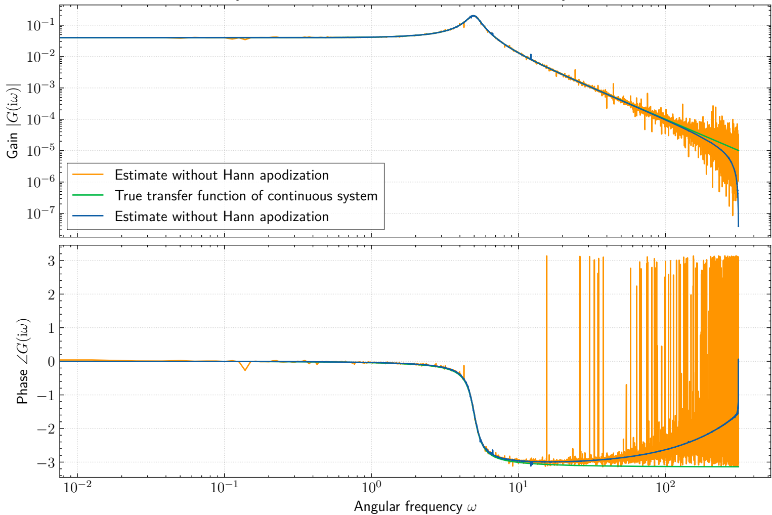
System identification of a second-order ZOH system
