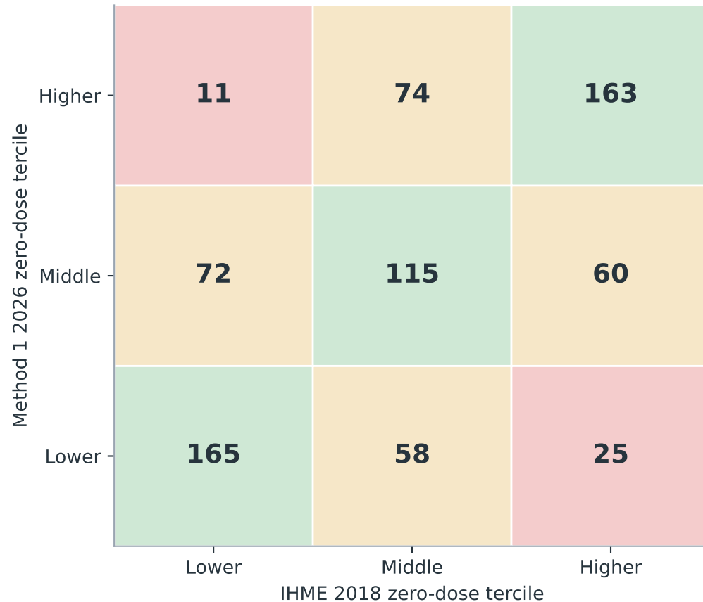
A. Tercile agreement: 443 same, 36 opposite
