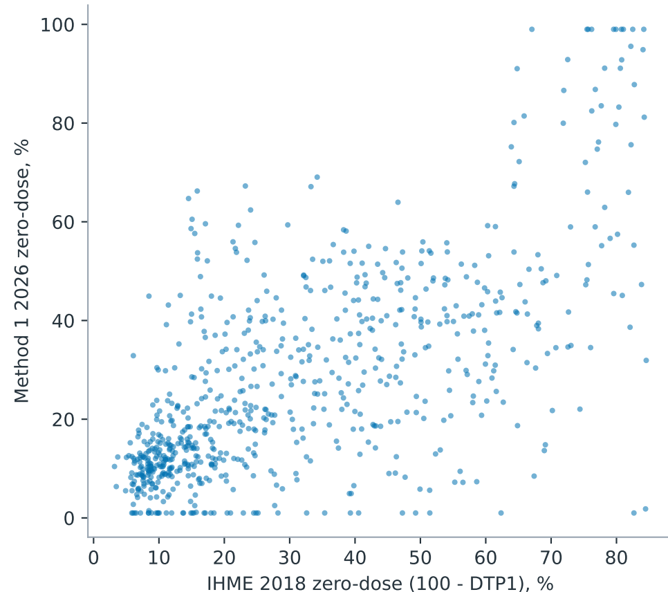
B. 743 LGAs: Spearman rho = 0.65 (95% CI 0.60-0.70)
